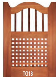
archtop dowel & lattice gates Size Cedar Kwila 1800 x 900 x 45 $1000 $1200 1300 x 900 x 45 $807 $969 1300 x 1400 x 45 $1066 $1280
