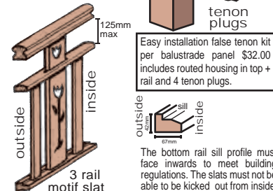
TB10 - 3 RAIL SLAT BALUSTRADE showing double motif center panel option
